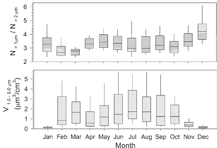
図8 粒子数濃度比 ( N_{>1\mu\text{m}}/N_{>2\mu\text{m}} ) と、粗大粒子体積濃度 ( V_{1.0-5.0\mu\text{m}} ) の季節変化。箱ひげ図の表し方はこれまでと同じ。 Fig. 8. Upper panel: seasonal variation of concentration ratios as N_{>1\mu\text{m}}/N_{>2\mu\text{m}} at Syowa Station. Lower panel: seasonal variation of volume concentration ( V_{1.0-5.0\mu\text{m}} ) in coarse size range.
