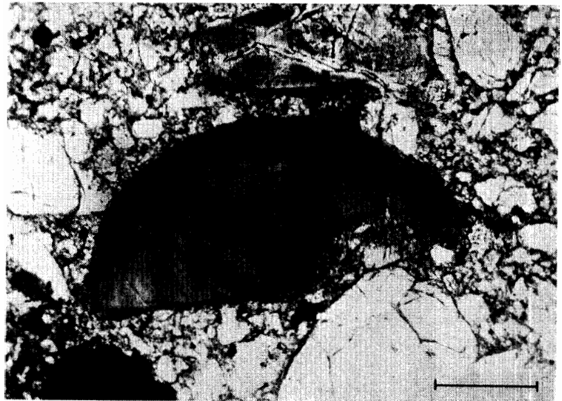
Fig. 13. A brown-colored spherule fragment composed of radial growth of fine acicular crystals in Yamato-7308. Minute metallic spherules are included. The bar is 0.2 mm in length.
