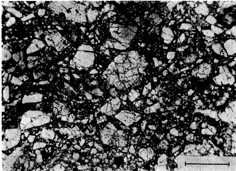
Fig. 4. Brecciated structure consisting of angular pyroxene and plagioclase grains in the matrix of Yamato-7308. The bar is 0.5 mm in length.
