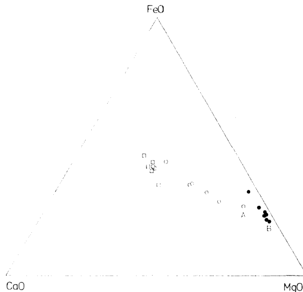
Fig. 17. CaO-FeO-MgO diagram of eucrites, howardites and diogenites.
