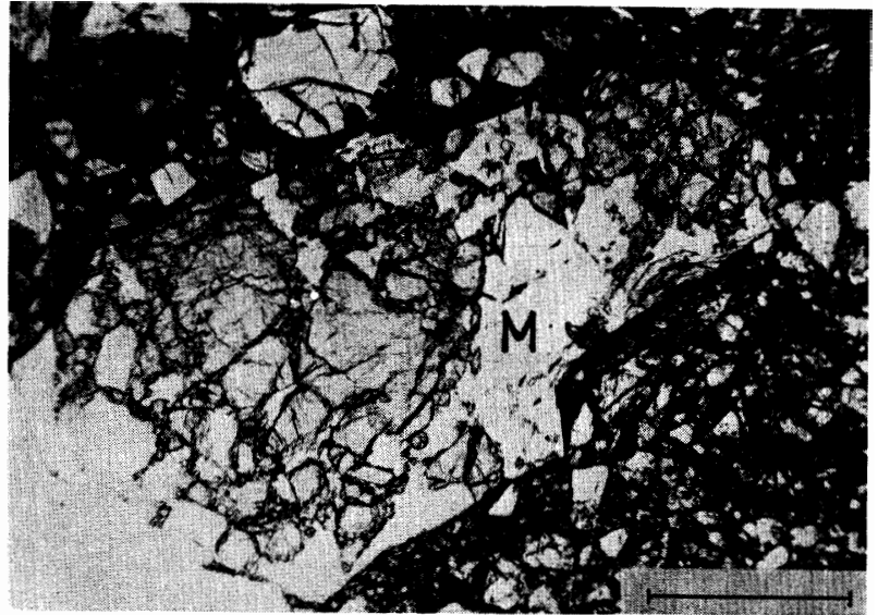
Fig. 12. Maskelynite (M) in the eucritic fragment of Yamato-7308. The bar is 0.5 mm in length.
