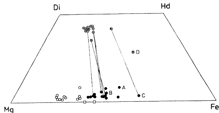
Fig. 18. Pyroxene composition of Yamato-7308.
