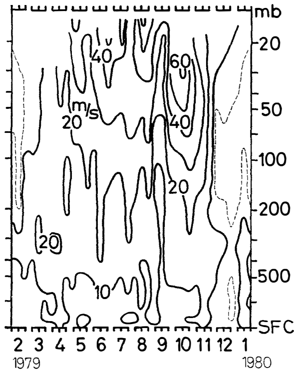
図 3 上層の旬平均風速の年変化図 Fig. 3. Annual variation of ten-day mean wind speed.
