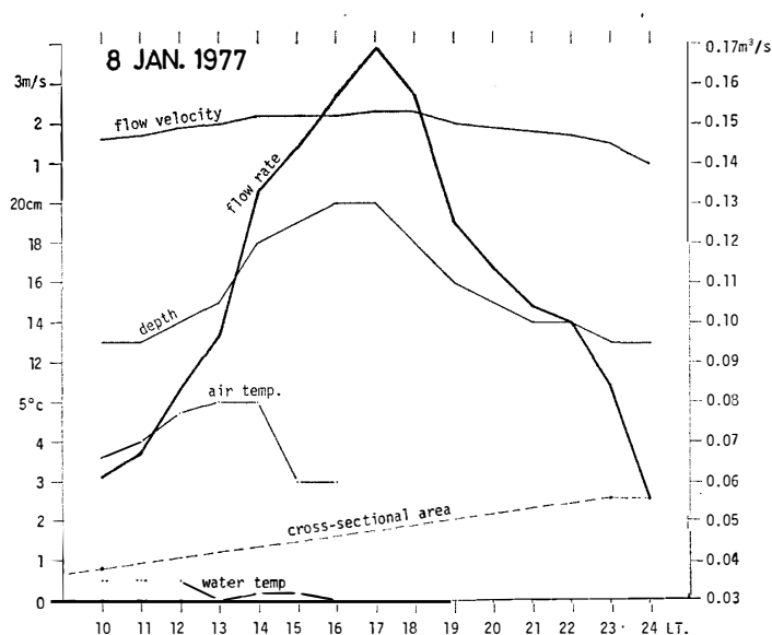
Fig. 12. Hourly change of amount of meltwater at the observation station (shown in Figs. 1 and 11). The flow rate ( V m 3 /s) at each hour was calculated from the following equation;
