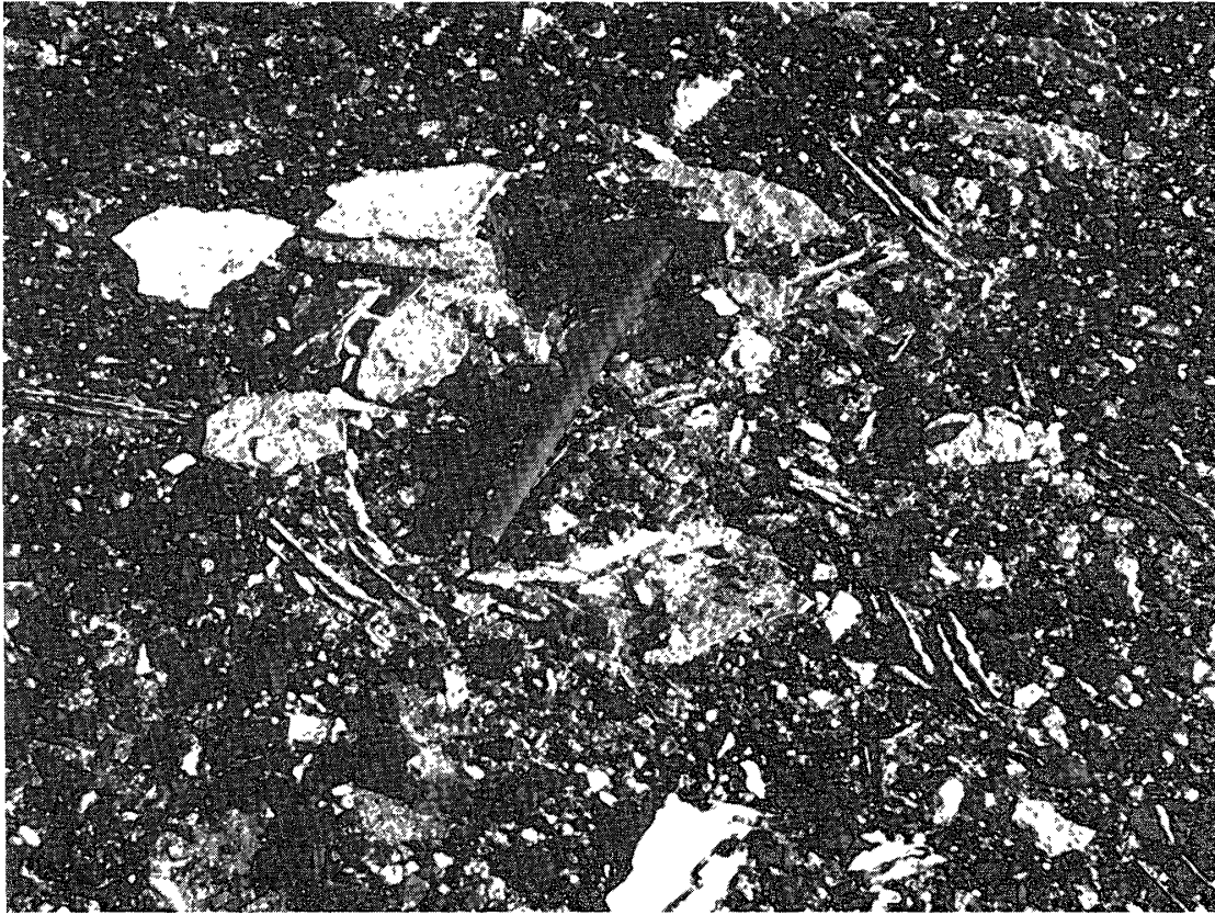
Photo. 3. Evaporites on the flat surface of moraine (near locality C in Fig. 2).
