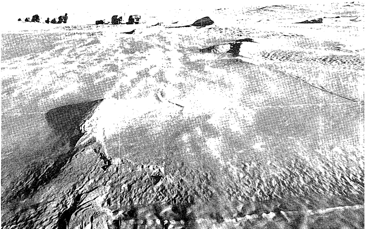
Photo. 4. Bare firn on the transverse step. Tortoise shell shape cracks show on the surface.
