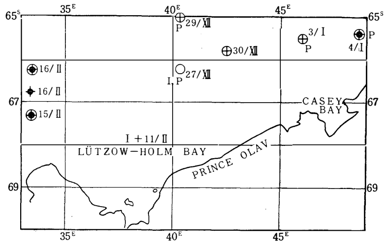
Fig. 3. Stations: vertical observation carried out.
