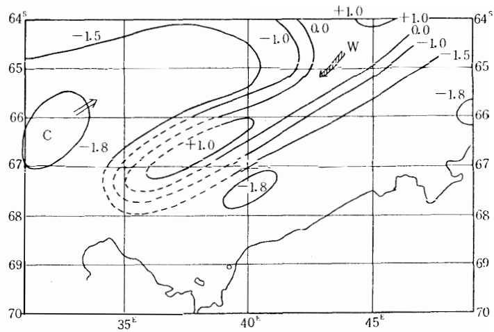
Fig. 14. Isotherm of 100 m depth.
