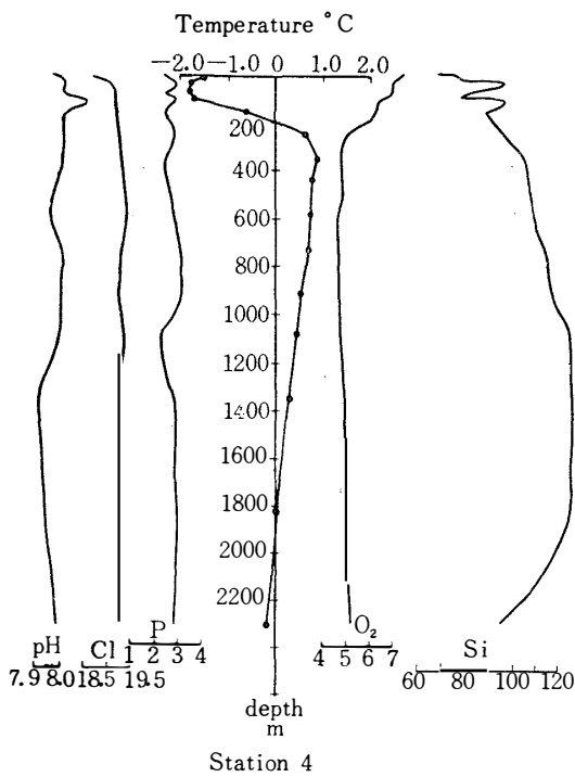
Fig. 7. Results of vertical observation. 3-I-1962 65°-26'S, 46°00'E
