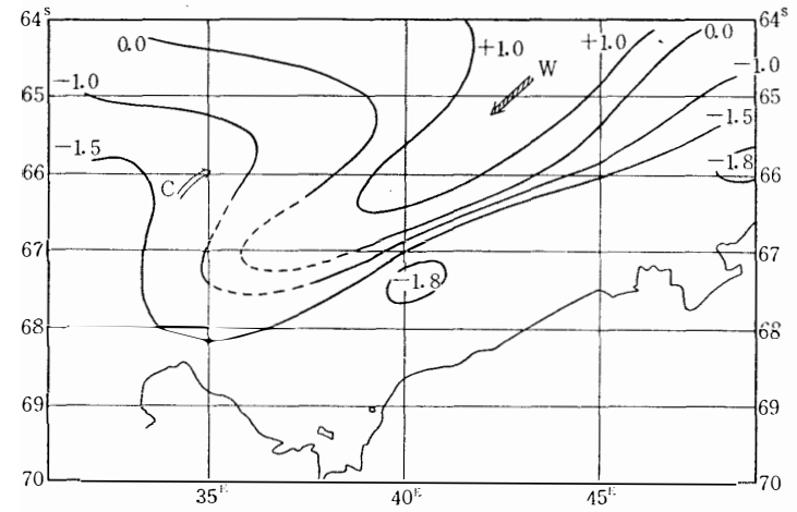
Fig. 15. Isotherm of 150 m depth.
