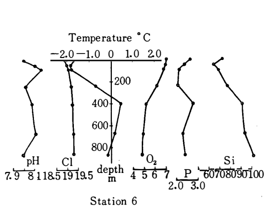
Fig. 9. Results of vertical observation. 15-II-1962 67°33'S, 33°35'E
