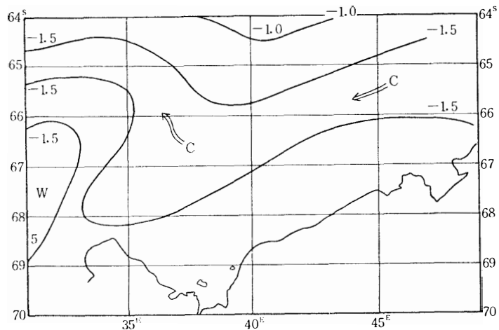
Fig. 13. Isotherm of 50 m depth.
