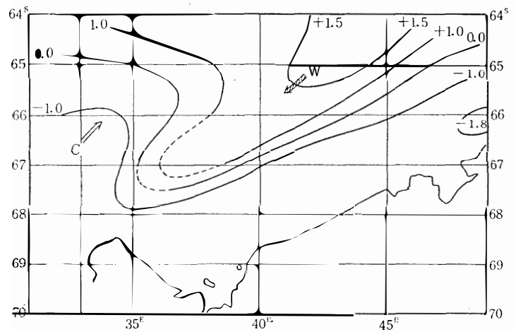
Fig. 16. Isotherm of 200 m depth.
