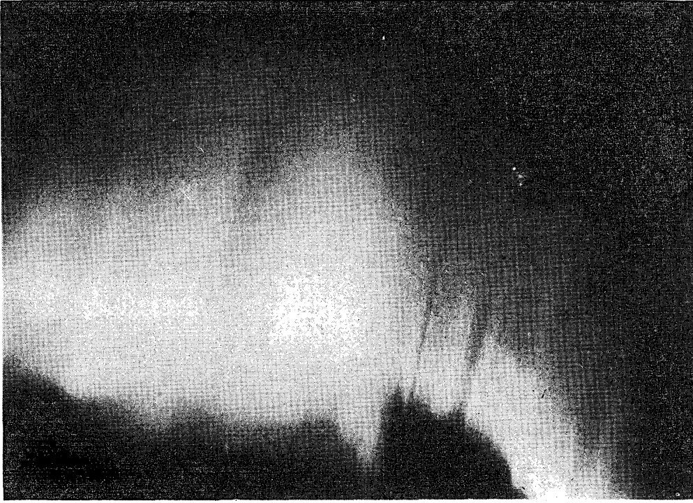
Ray Bundle. 23 : 25, Mar. 26, 1959.
