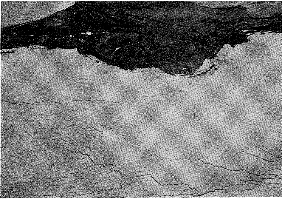
Surface of the ice-sheet eroded by melted water (1).
