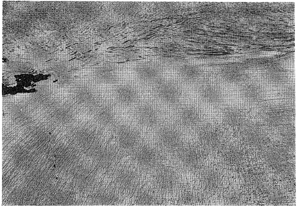
Surface of the ice-sheet eroded by melted water (2).
