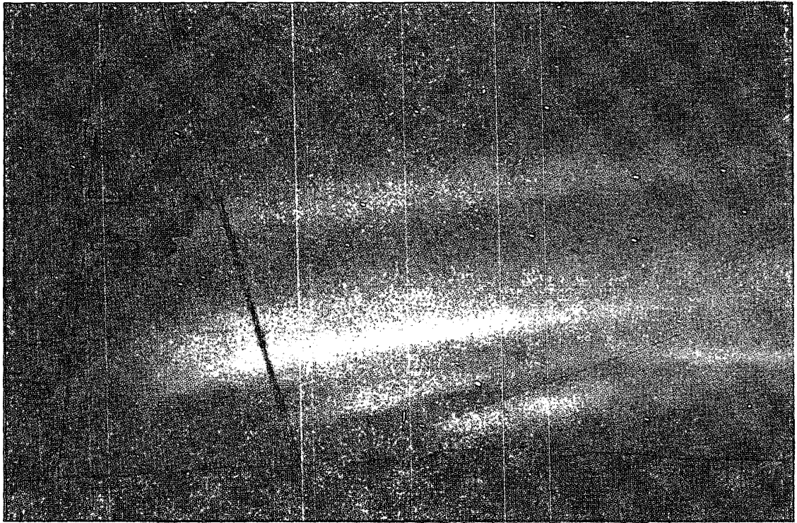
An aspect of auroral activity immediately before its climax.
