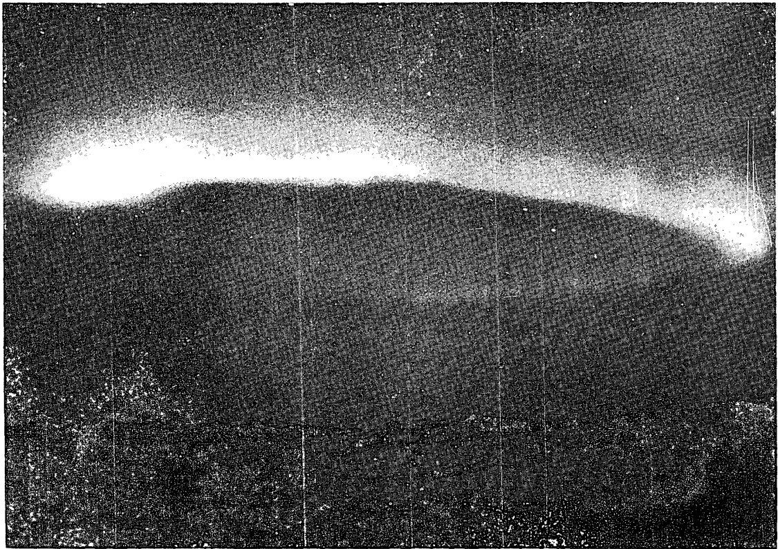
Crown type aurora: a kind of draperies.
