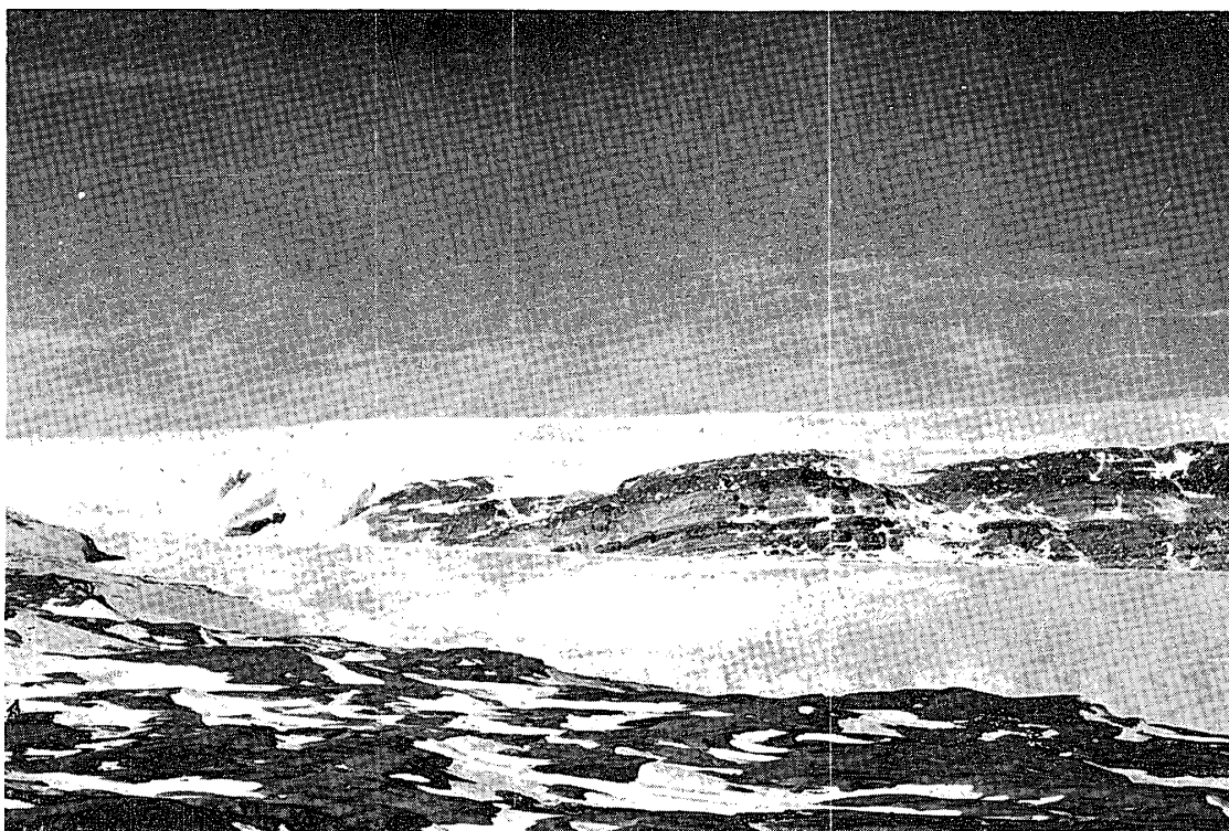
An ice fall at the margin of the inland ice, on the southern coast of Skallevika. The height of the horizon of the inland ice is about 200 meters. (taken by T. Tatsumi on October 26, 1957)
