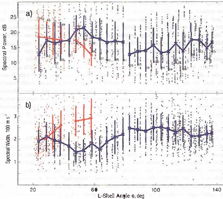
Fig. 10. Spectral power at HF versus Lshell angle for 0100–0130 UT on March 17, 1997, panel (a). Red (blue) points are echoes with velocity magnitude larger (smaller) than V_{crit} = 320 \text{ ms}^{-1} . Averaged (for 5^\circ -wide bins in Lshell angle) values, standard deviations and numbers of points are indicated for high- and low-velocity HF echoes. The spectral width at HF versus L-shell angle is shown in panel (b).
