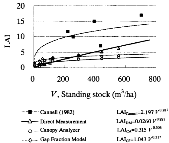
Fig. 12. Comparison among four different relationship between LAI and standing stock in conifers.
