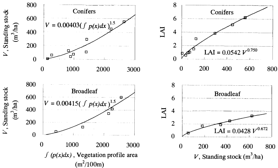
Fig. 8. Relationship between standing stock and LAI.
