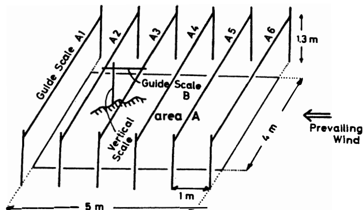
Fig. 2. Measuring system of the level of the snow surface.
