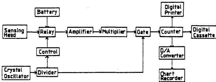
Fig. 2. Schematic illustration of the data acquisition system. The upper figure shows the device constitution and the lower figure does the block diagram.
