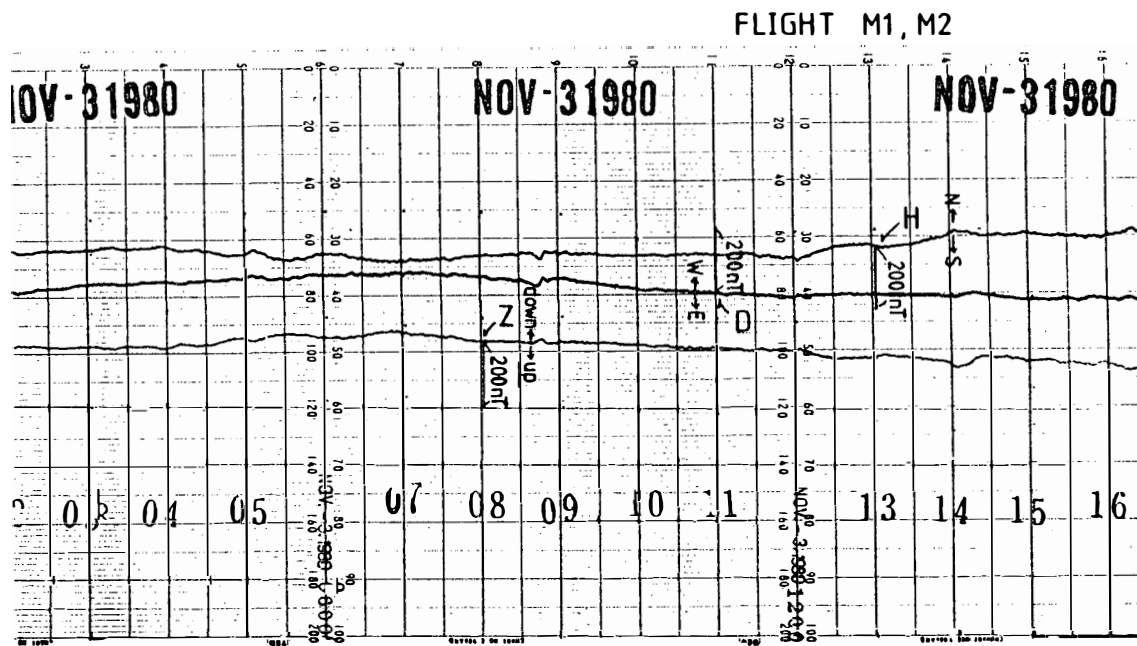
Fig. 5. Monitor records of diurnal variations of three-component (H, D, Z) geomagnetic field for the 5 flights in Table 3.
