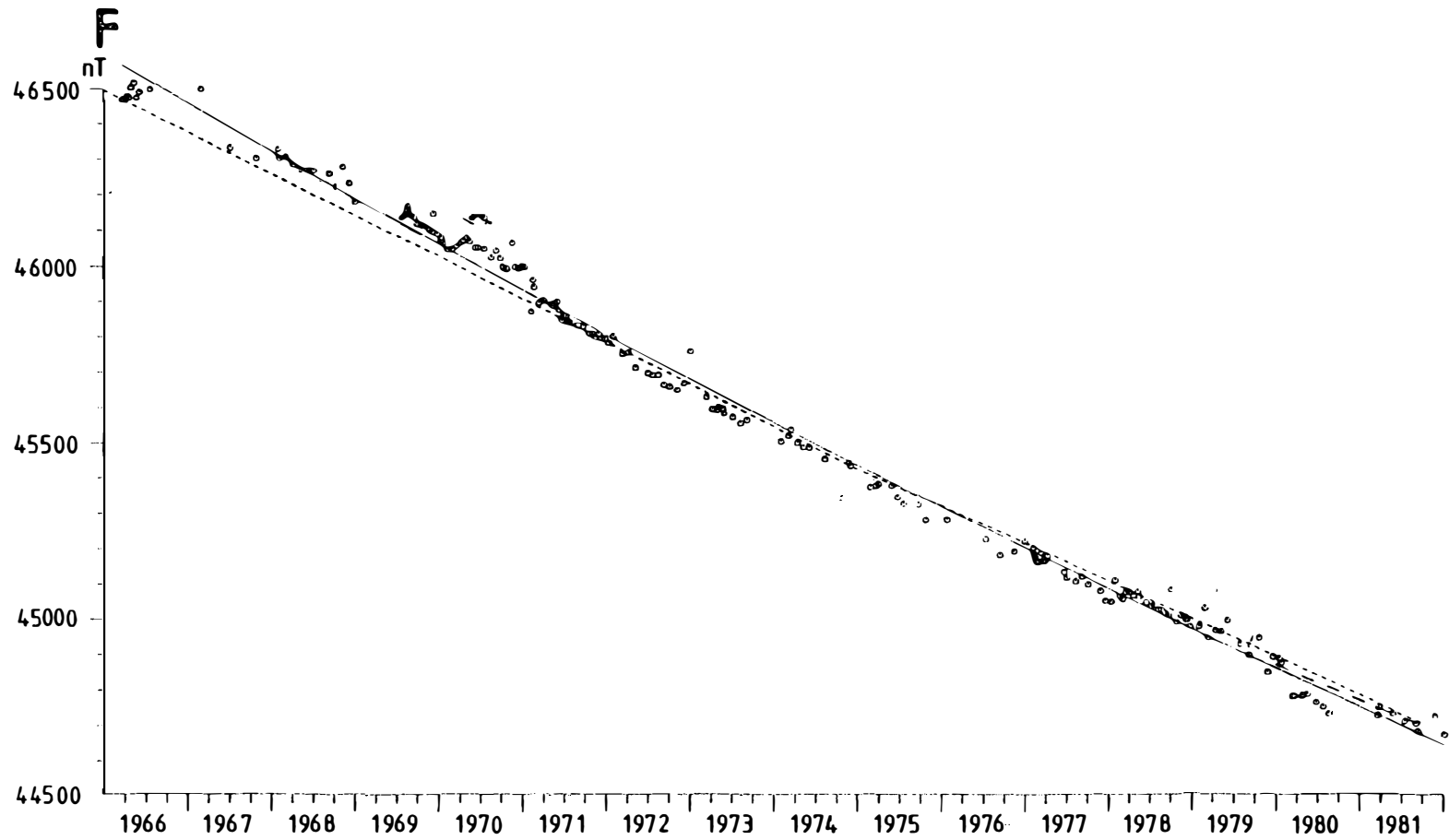
Fig. 4. Secular variation of the geomagnetic total intensity at Syowa Station, reproduced from Shibuya and Tanaka (1983).
