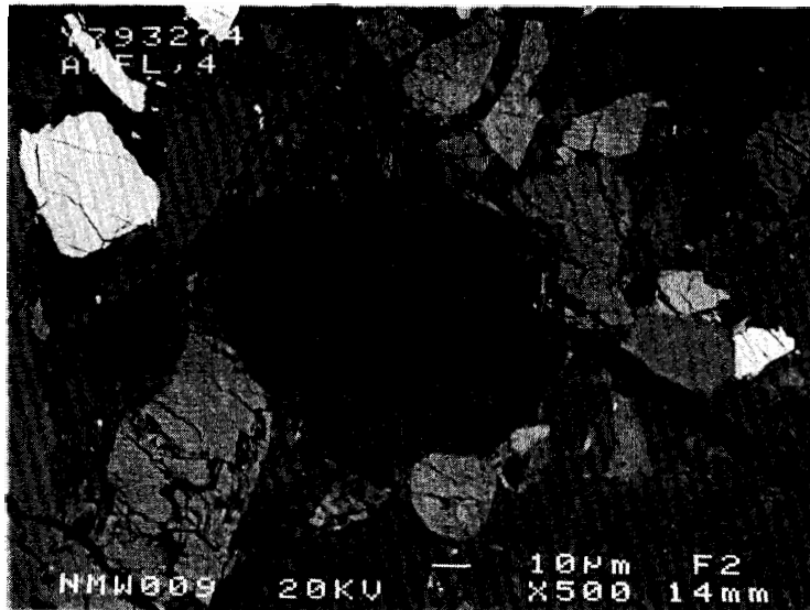
Fig. 11. BSE image of an intergrowth of silica (dark gray) and K-feldspar (lighter gray) in sample ,93.
