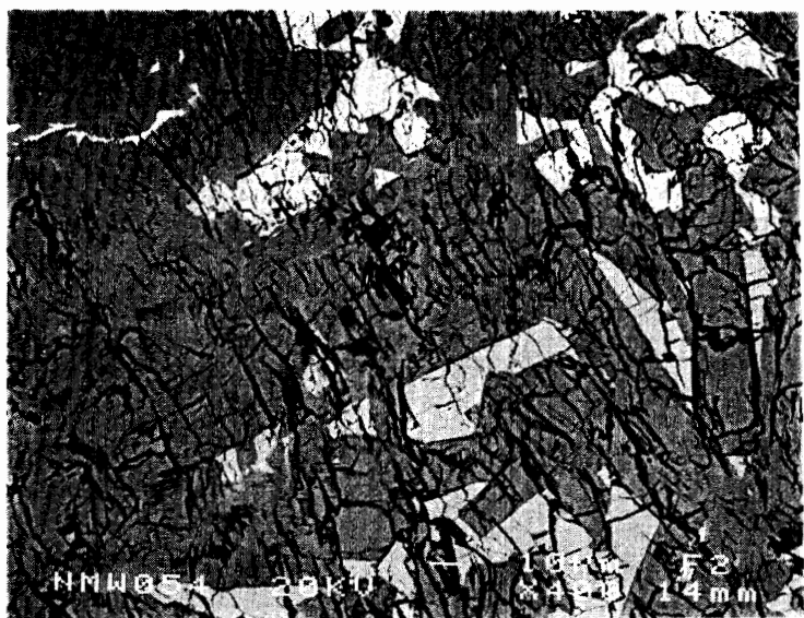
Fig. 13. BSE image of a meta-anorthositic gabbro clast from sample ,93 (part of clast WC2, see Table 5 for trace element data). The light gray ferromagnesian mineral in the upper part of the image is olivine, while the slightly darker mineral in the lower part is pyroxene.
