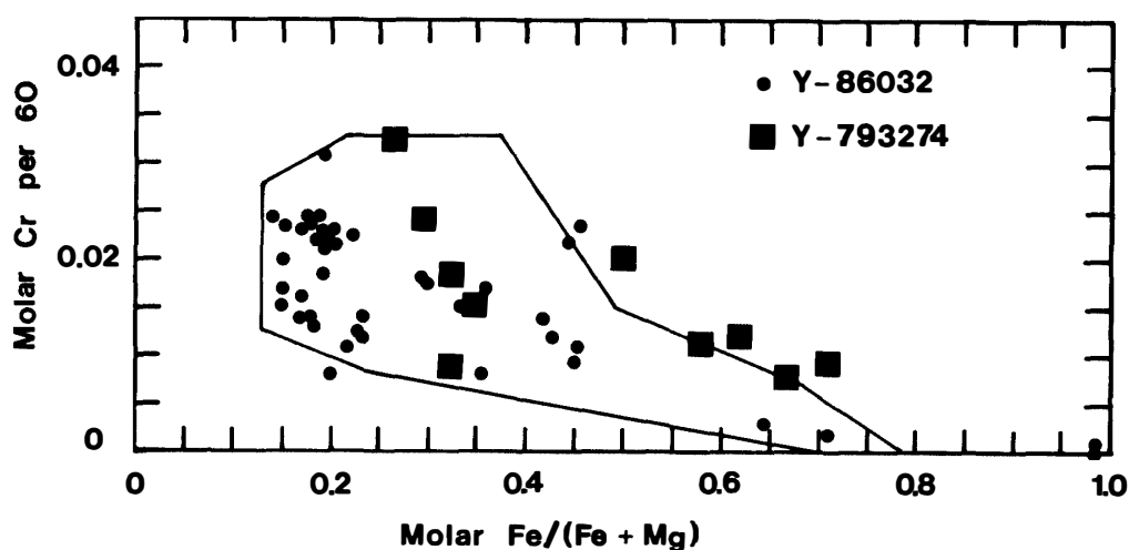
Fig. 9. Molar Cr in Y-793274 pyroxenes vs. molar Fe/(Fe+Mg) ratio, compared to highlands breccia Y-86032, obtained by electron probe microanalysis. The Fe-rich pyroxenes plot partly outside the field defined by highland pyroxene compositions (see, e. g., KOEBERL et al., 1990b), indicating the presence of mare components.
