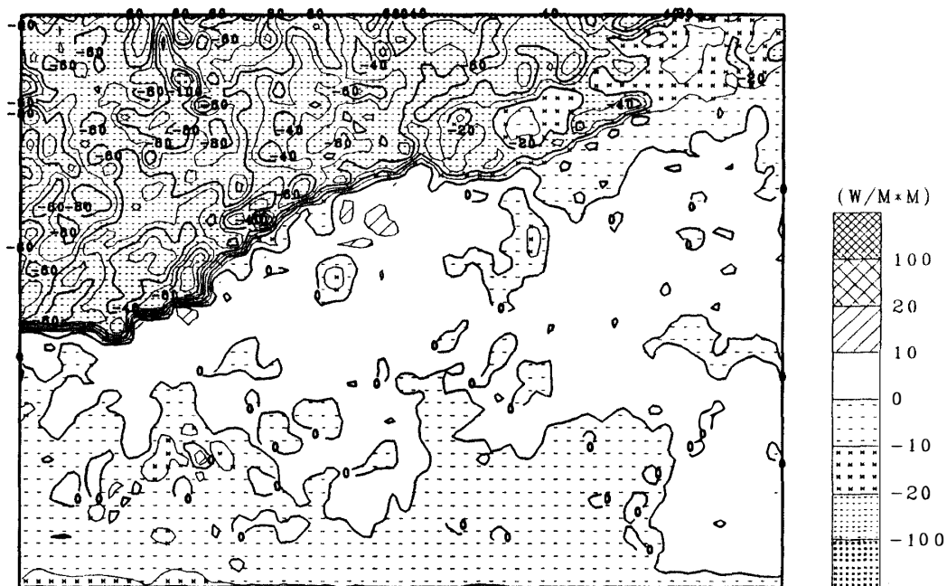
Fig. 7. Shortwave cloud-radiative forcing ( W/m^2 ) at the top of the atmosphere in the area shown in Fig. 1 in December 1988.
