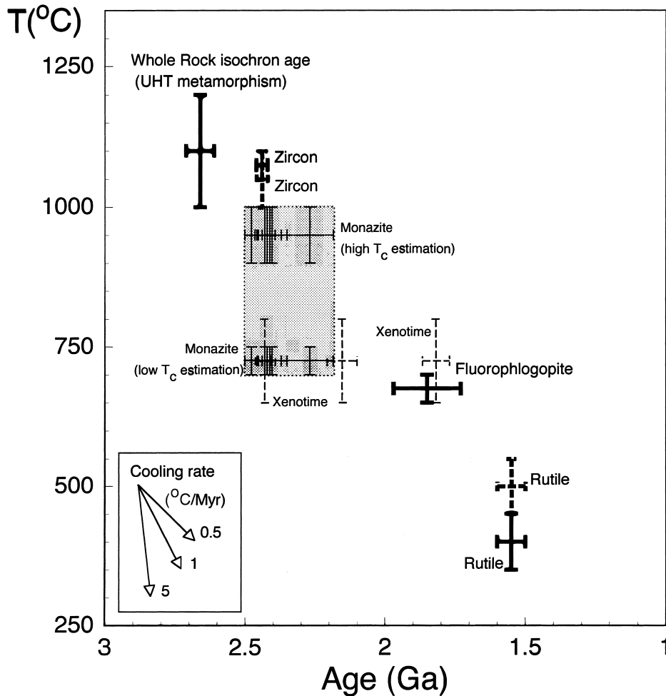
Fig. 8. Apparent temperature-time ( T - t ) relation for metamorphic rocks from the Howard Hills. Age data are taken from the result of this study and Miyamoto et al. (2004). The Sm-Nd whole-rock isochron age is regarded as the time of peak metamorphism for the dated sample (Miyamoto et al., 2004). The metamorphic temperature (1000°–1200°C) is quoted from Yoshimura et al. (2000). Estimations of closure temperatures for each mineral are as follows: 1050°–1100°C for closure temperature of zircon age (Cliff, 1985); 650°–700°C for fluorophlogopite under dry condition (Kühn et al., 2000); 350°–450°C for rutile age (Mezger et al., 1989), and based on diffusion parameters (thick and broken lines): 1000°–1100°C for zircon (Cherniak and Watson, 2000); 450°–550°C for rutile (Cherniak, 2000). The Th-U-Pb CHIME ages for monazite and xenotime are obtained from Grew et al. (2001), Asami et al. (2002), and Suzuki et al. (2006). Their temperature estimations are based on the diffusion parameter: 700°–750°C for monazite (Parrish, 1990; low T_c estimation in the figure) and 900°–1000°C for monazite (Cherniak et al., 2004, high T_c estimation in the figure); 650°–800°C for xenotime (Heaman and Parrish, 1991; Kamber et al., 1998). The shaded square is an area of T - t points for monazite.
