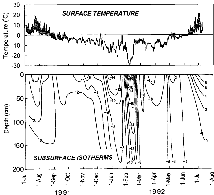
Fig 8 Annual variation in ground temperature at the KL site Isotherm intervals are 2^{\circ}\text{C} The dotted area represents the active layer The triangle indicates the depth of the frost table confirmed by excavation
