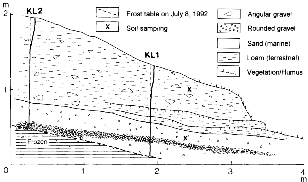
Fig 3 The longitudinal section of the frontal part of a solifluction sheet at the KL site, showing deformation of strain probes (KL1 and KL2) over two years
