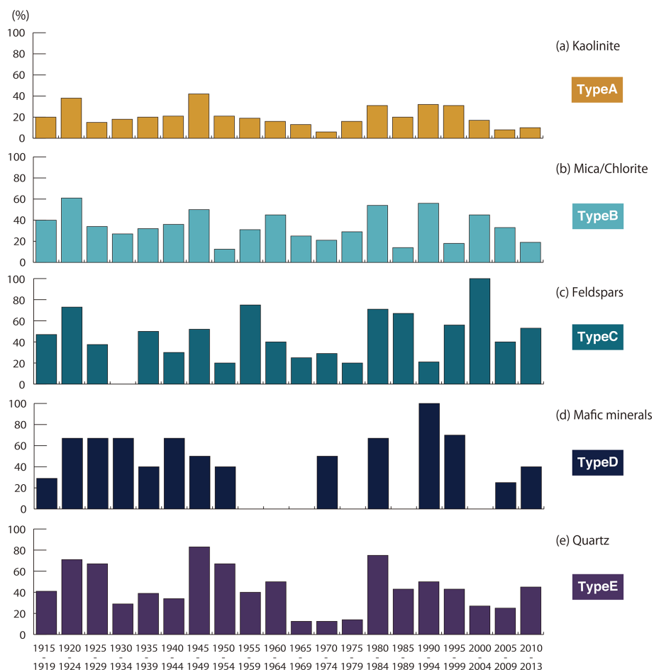
Figure 10. Historical changes in proportion of large particles (diameter > 2 μm) in (a) kaolinite, (b) mica–chlorite, (c) feldspars, (d) mafic minerals, and (e) quartz.
