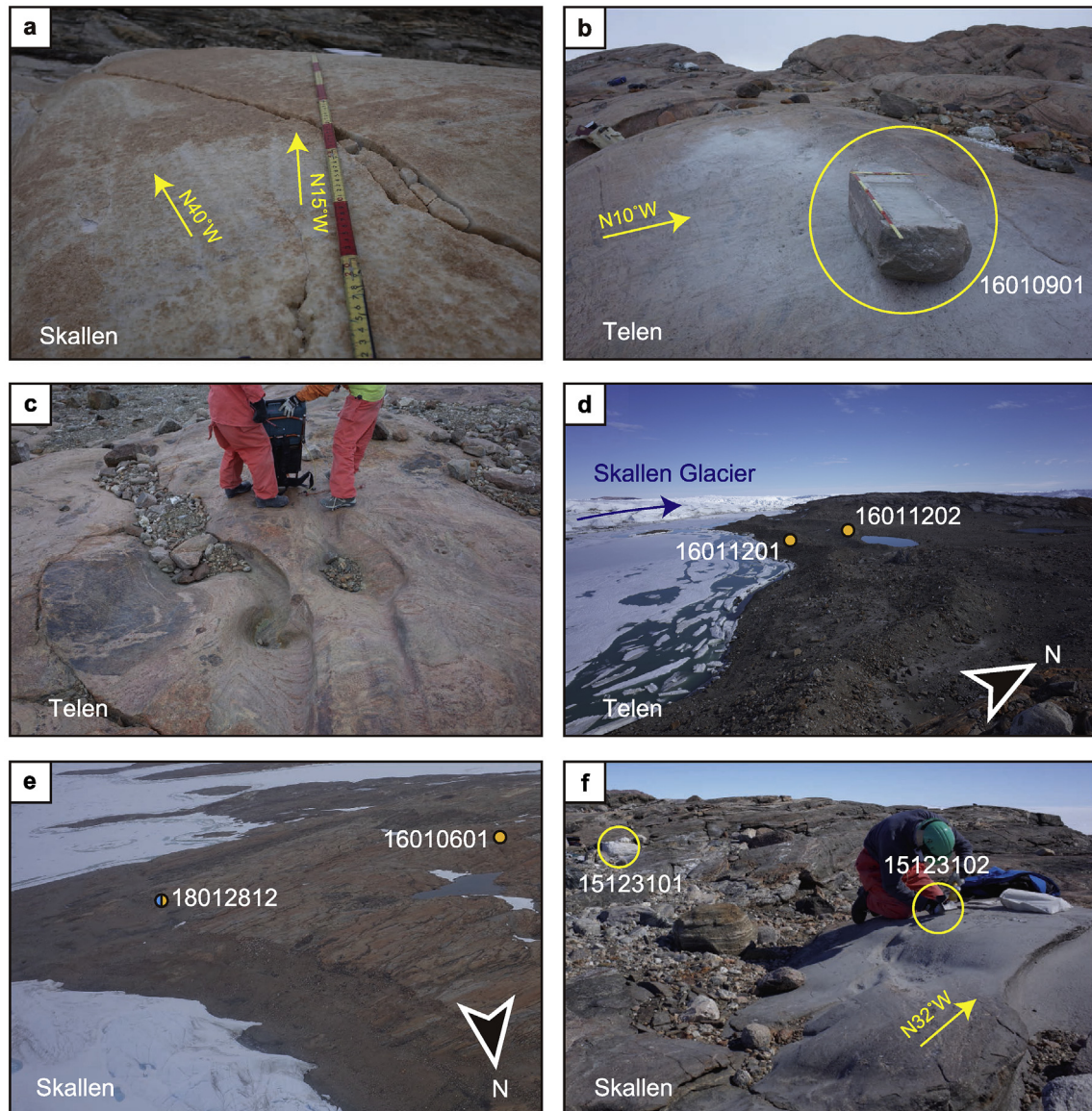
Fig. 7. Glacial geomorphology at Skallen and Telen. Localities are shown in Figs. 2 and 3. (a) N15°W striations cross-cutting N40°W striations at Skallen. (b) Sampling site 16010901 at Telen. (c) Sculpted erosional form at Telen. This form indicates a subglacial meltwater flow event (Sawagaki and Hirakawa, 1997). (d) Lateral moraines flanking Skallen Glacier at Telen. (e) Bird's eye view looking from the northeastern side of Skallen. (f) Bedrock sampling at Skallen, showing unweathered and smooth bedrock. Yellow circles and arrows show samples for dating and orientations of striations, respectively. (For interpretation of the references to colour in this figure legend, the reader is referred to the Web version of this article.)
