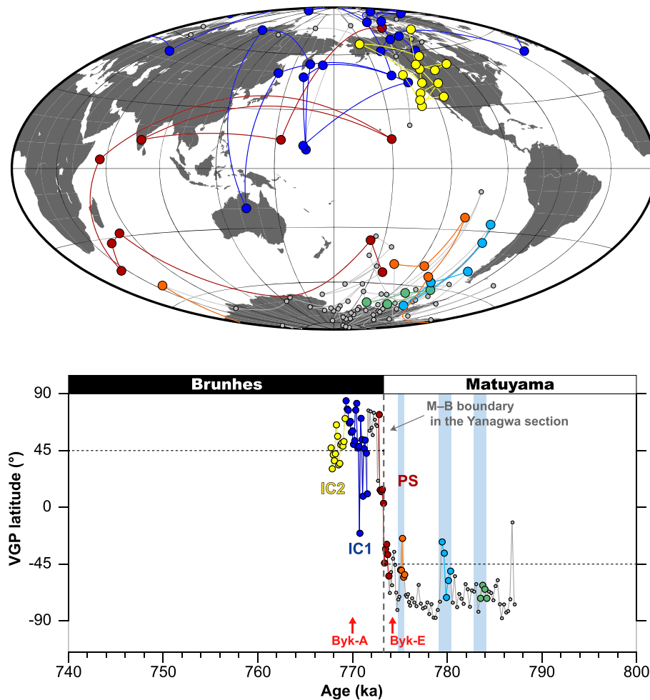
Fig. 11 VGP paths (top plot) and time evolution of the VGP latitude (bottom plot) from the Chiba and Yanagawa sections. Data are based on the progressive thermal demagnetization of Suganuma et al. (2015). The temporal profile was calculated from the most recent age model of Suganuma et al. (2018). Blue vertical shades and gray vertical dashed line indicate millennial-scale VGP fluctuations and the M-B boundary, respectively. Ages of the Byk-A and Byk-E tephra beds are indicated by red arrows. IC, instability cluster; PS, polarity switch
