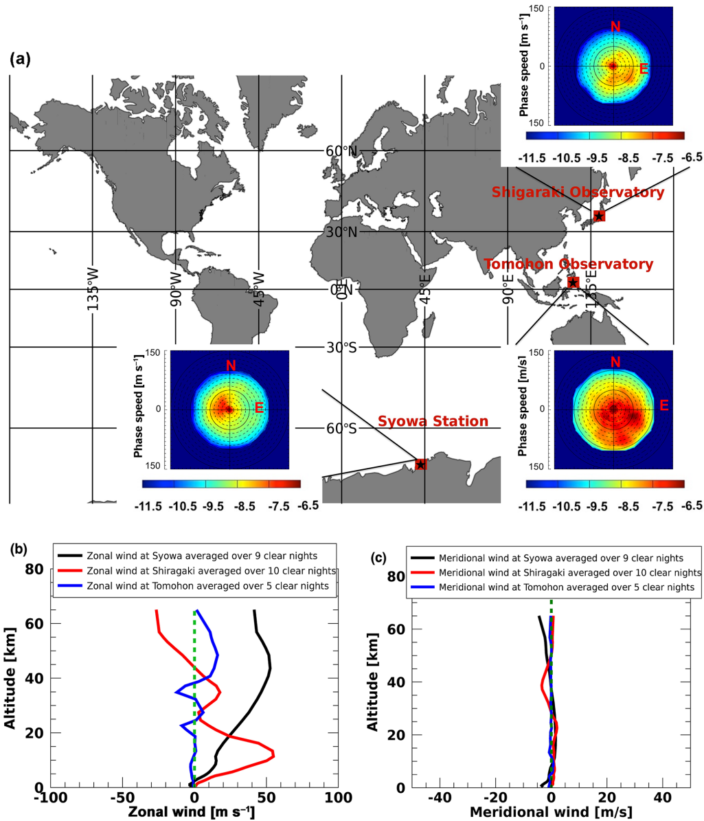
Figure 4. (a) Average day-to-day variation of the 2-D phase velocity spectrum of AGWs observed at Syowa, in Shigaraki, and in Tomohon. (b) Average zonal wind profiles (positive: eastward) and (c) average meridional wind profiles (positive: northward) of GWs observed during clear nights from MERRA-2 data.
