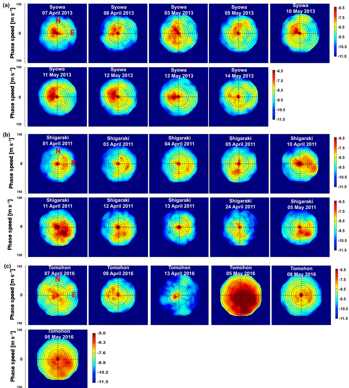
Figure 3. Day-to-day variation of 2-D phase velocity spectra for April–May 2013 at the Syowa Station (a), in Shigaraki (2011) (b), and in Tomohon (2016) (c). Panel (c) is the same as that for 5 May 2016, but with a different color bar level to better visualize the dominant wave propagation direction.
