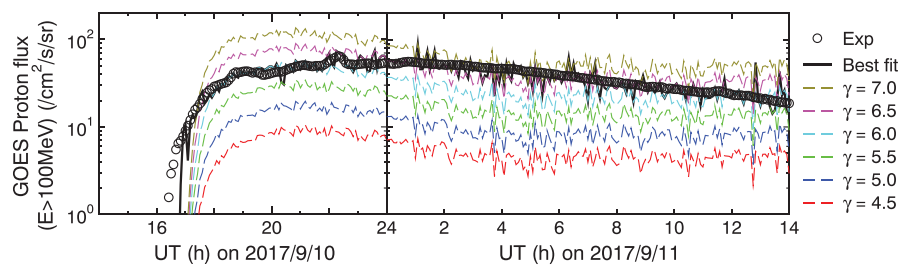
Figure 2. Proton flux at >100 MeV as measured by the GOES satellites (circles), compared against our calculated data (dashed curves) obtained by varying the power-law spectral index \gamma of the injected protons from 4.5 to 7.0.
