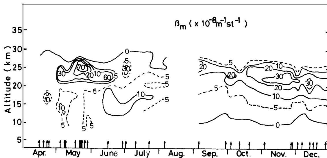
Fig. 2. The time-height cross section of particulate backscattering coefficient during the period of April to December 1982.
