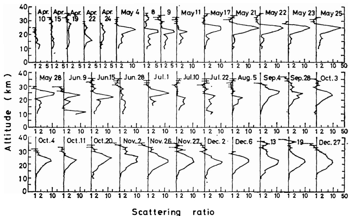
Fig. 1b. The scattering ratio profiles from April to December 1982. Error was shown by "—".
