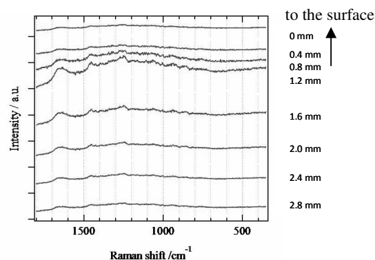
Figure 1. The depth dependence of Raman spectral change of a bovine cornea measured by a portable Raman spectrophotometer.
