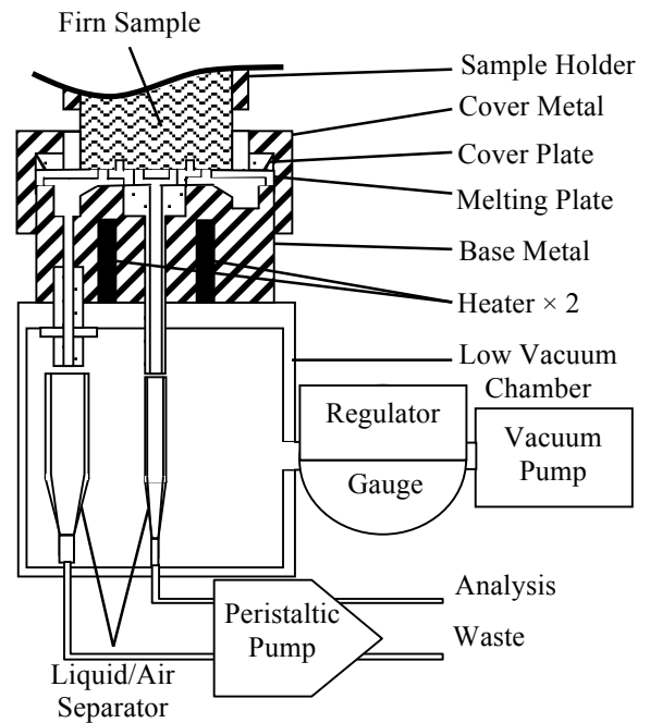
Figure1. Melting system
