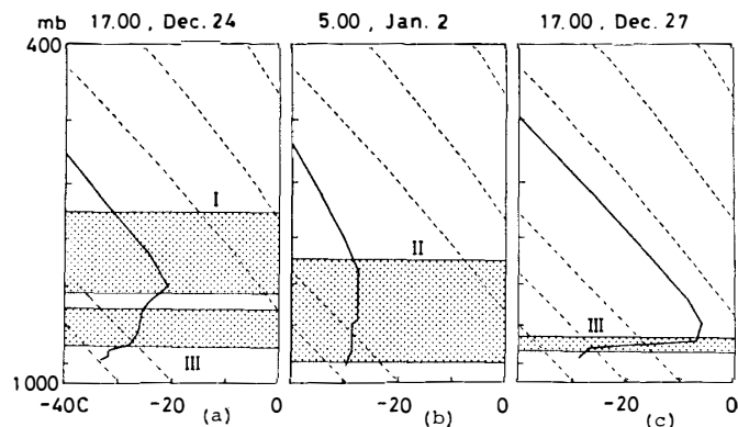
Fig. 4. Three types of vertical profiles of temperature in cloud layer which is shown by shaded area.
