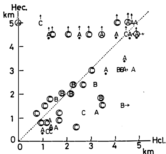
Fig. 9. Difference between the levels of cloud top ( H_{cl} ) and echo top ( H_{ec} ). Letters A, B and C correspond to periods A, B and C, respectively. Vertical and horizontal arrows indicate that H_{ec} and H_{cl} might be underestimated because of the limitation of radar and sounding systems, respectively. Letters with dots and encircled letters mean that rimed crystals and snow crystals of peculiar shape were observed, respectively.
