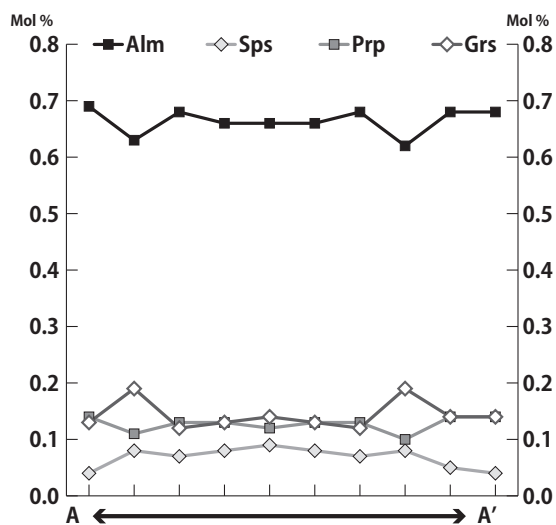
Fig. 2. Plots of garnet zoning profiles for the grain showing in Fig. 2.
