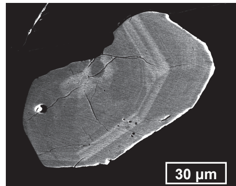
Fig. 3. Back scattered electron image of zircon in garnet amphibolite. Zircon grains have oscillatory zoned igneous cores and structureless rims which are probably of metamorphic origin.
