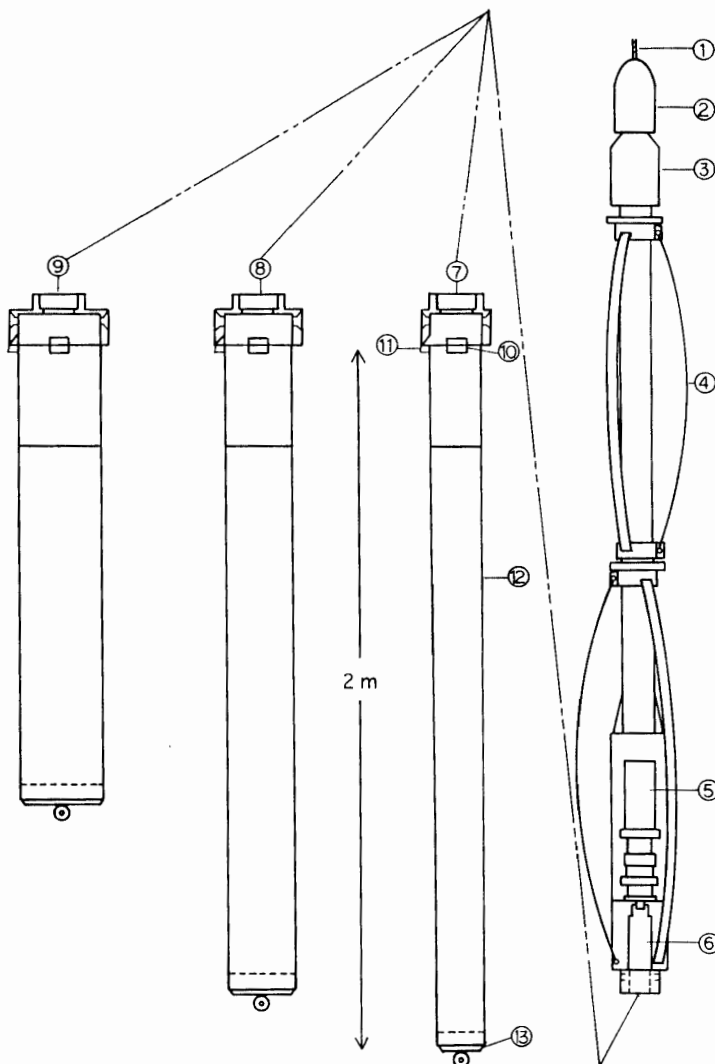
Fig. 4. Cross-sectional drawing of the electro-mechanical reamer.
