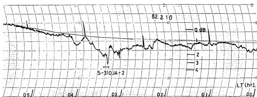
図 2 30 MHz リオメータ記録 (00 h-05 h LT; February 10, 1977) (OSE et al. , 1978) Fig. 2. Riometer record of 30 MHz cosmic noise.
