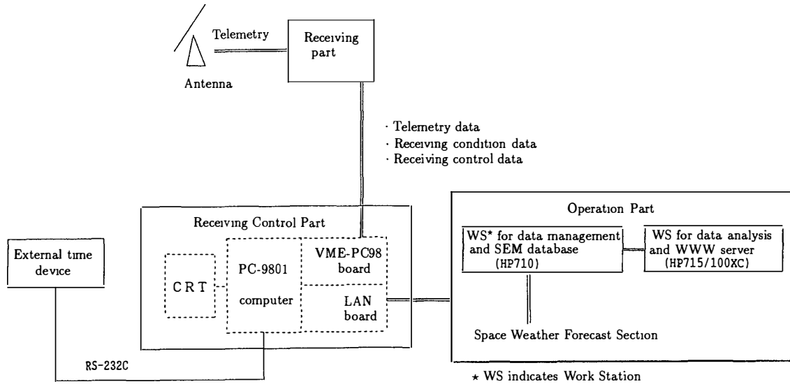
Fig. 1. Organization of the data acquisition system from GMS/SEM.
