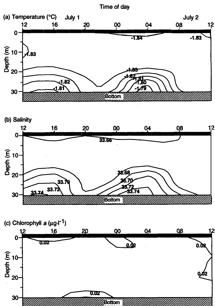
Fig. 2. Diel variation in vertical distribution of temperature (a), salinity (b) and chlorophyll a (c) at Stn. K during the period from 1200 LT, 1 July to 1200, 2 July in 1993. Black bars represent darkness throughout the investigation period.
