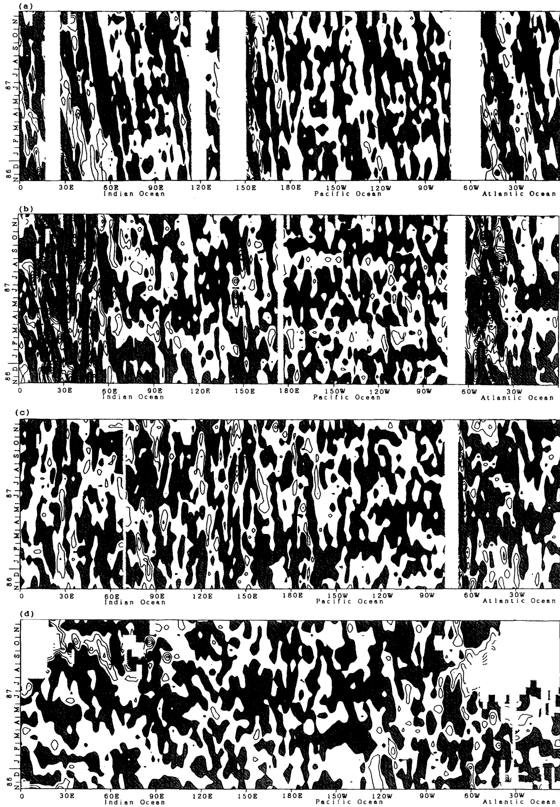
Fig. 5. The time-longitude dependency in sea-level anomaly at (a) 34°S, (b) 40°S, (c) 50°S and (d) 60°S. The contour interval is 5 cm. Hatched regions indicate the negative sea-level anomaly.
