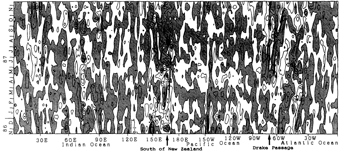
Fig. 4. The time-longitude dependency in sea-level anomaly along the line of 10.5 \text{ m}^2/\text{s}^2 in geopotential anomaly. The contour interval is 5 cm. Hatched regions indicate the negative sea level anomaly.
