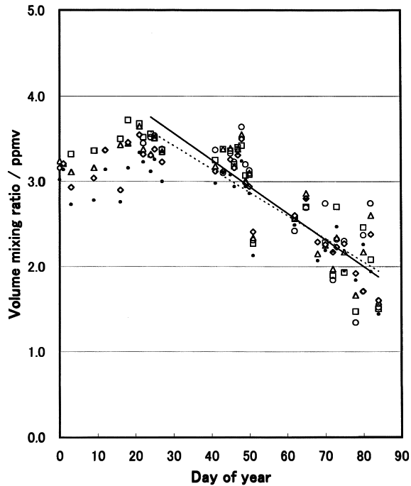
Fig. 11. Ozone mixing ratio (ppmv) in the air parcel that departed the 487 K isentropes on 31 December (day 0 of 1997), continued to diabatically descend, and reached the 470 K isentropes on 25 March (day 84 of 1997), together with those from 480 K to 440 K on 25 March inside the polar vortex over Eureka. The same symbols as in Fig. 7 are used. Solid (dotted) lines indicate linear decreasing trends from 24 January to 25 March for 470 K (450 K).
