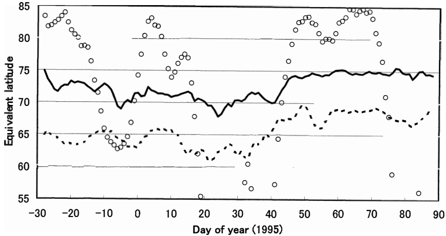
Fig. 1. Equivalent latitudes of the polar vortex boundary region and Eureka on the 475 K isentrope in the Northern Hemisphere in 1994/95. Solid (dashed) lines indicate the poleward (equatorward) edges of the boundary region of the polar vortex. The circles indicate Eureka. The data shown were smoothed in time with a 5-day running mean.
