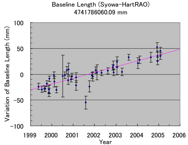
Figure 2. Variation of Baseline Length (Syowa-HartRAO)
