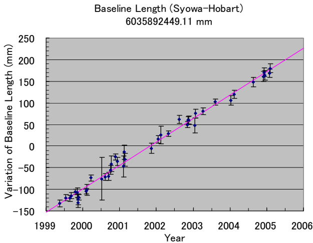
Figure 1. Variation of Baseline Length (Syowa-Hobart)
