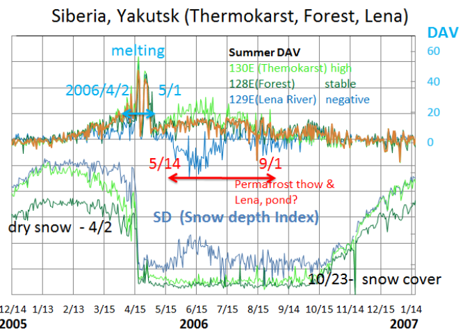
図4. 森林、氾濫原、サーモカルストのマイクロ波日サイクルの変化 (DAV)。DAVの融雪後の地域差。 Figure 4. Diurnal variation of microwave signals from forest, flood area and thermokarst area. Snow melting is apparent. After snow melting, the diurnal signal shows different regional characteristics.
