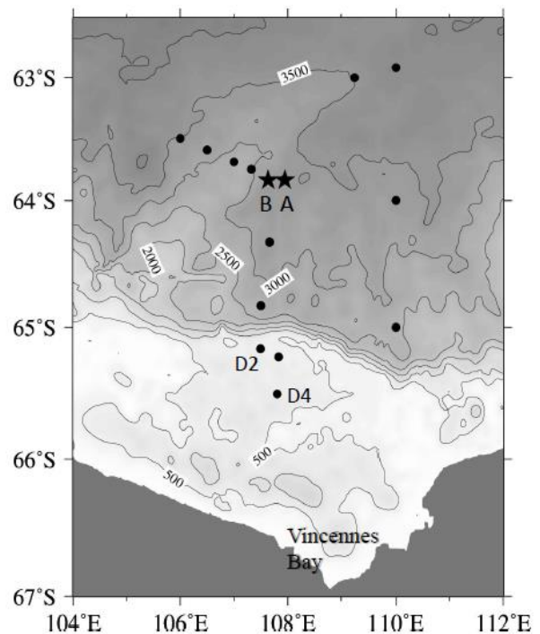
Fig. 1. Locations of two mooring stations and CTD stations off Vincennes Bay. Mooring locations A and B are indicated by stars. CTD stations in 2014 are indicated by black dot.
